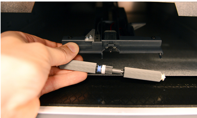
3. Remove pick-up roller
